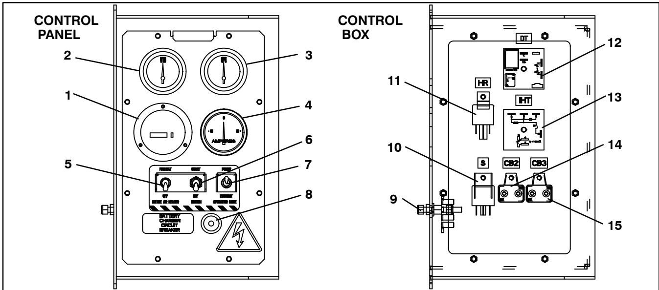
Figure 1-7 Standard Control Panel and Box With Dual Speed Option
