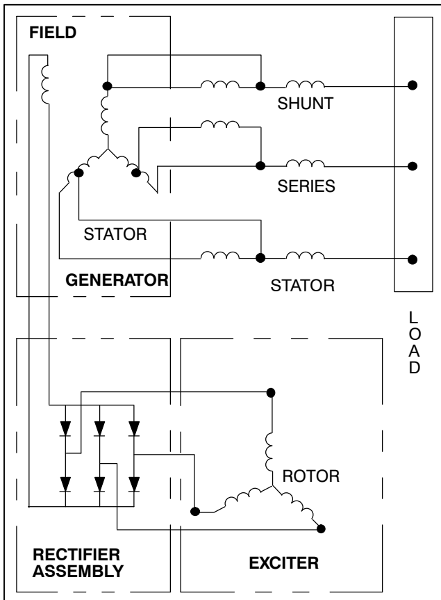
Figure 1-6 A-C Generator Circuit Diagram
