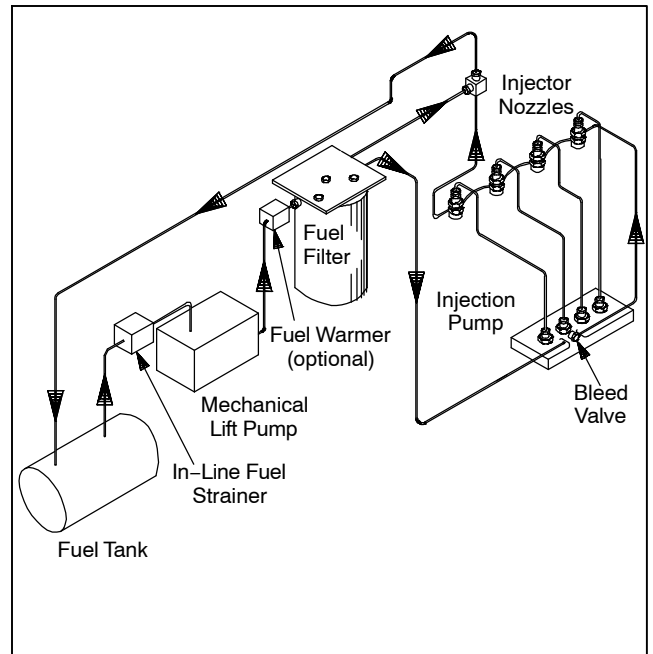
Figure 1-4 Fuel System Diagram
